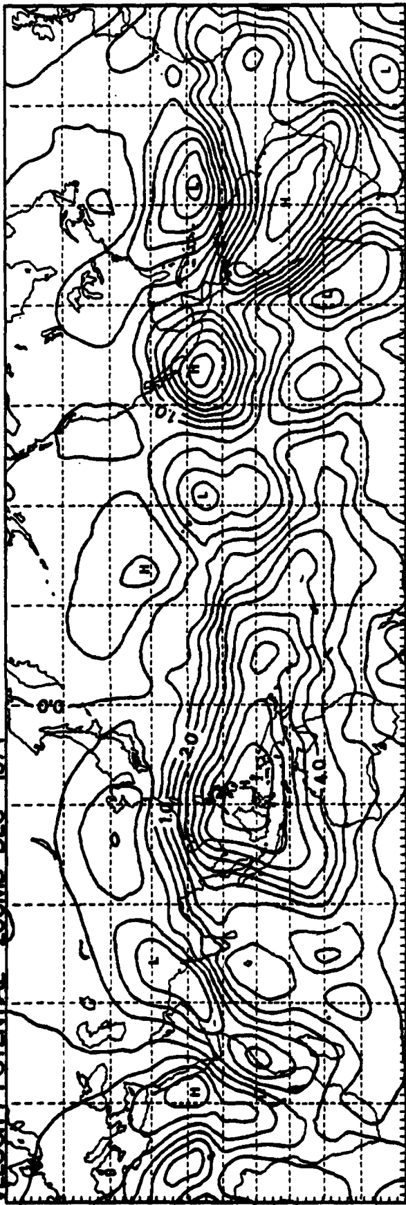
VELOCITY POTENTIAL 200MB DEC 1974
